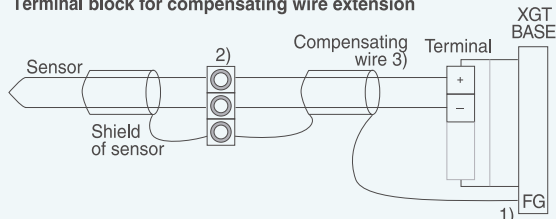
Terminal block for compensating wire extension
