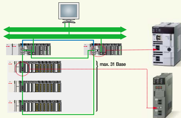
XGL-EIMT : Twisted pair 2ports For PC
